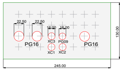
Bottom connections plate
