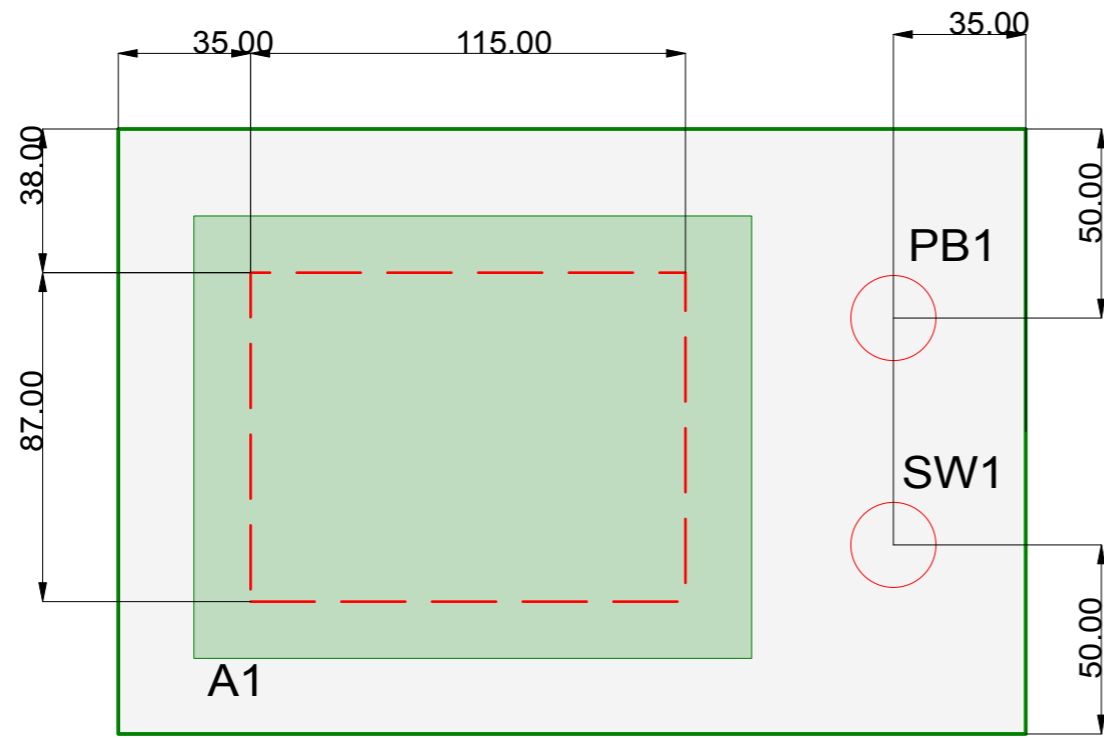
Front view
