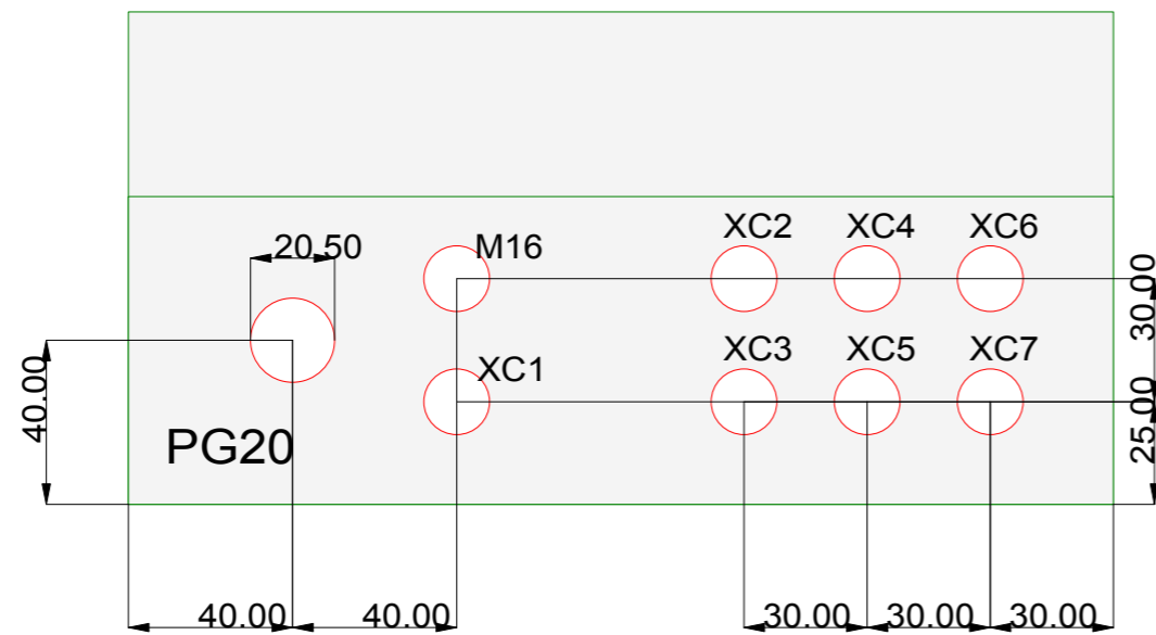
Bottom view
